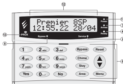
Premier LCD/LCDL/LCDP/LCDLP
